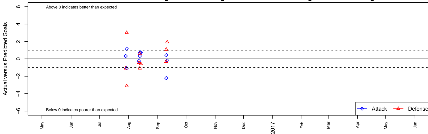
Spokane Sounders B B05 Dots are actual minus expected GF (blue circles) and GA (red triangles). Blue line is smoothed change in attack strength. Red is smoothed change in defense strength.
